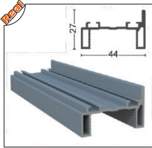
ISICM31-1010 Küçük h Fitol Contalı Esp.Handle Seal (With PVC Seal)
