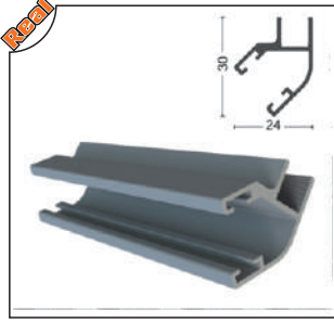
ALMFTL-1003 135° Fitil 135° Seal
