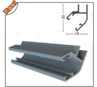
ALMFTL-1003 135° Fitiil Aluminum 135° Seal
