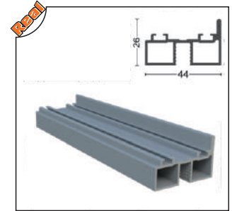
PRGLD-1004 Küçük h Fitil Contalı Aluminum Small 'h' Seal(With PVC Seal)
