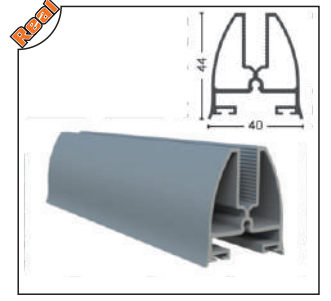
GLD-1003 Baza Profili Aluminum Glass Profile
