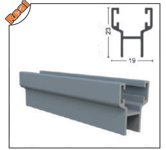
ALMFTL-1002 Büyük H Fitiil Big H Seal
