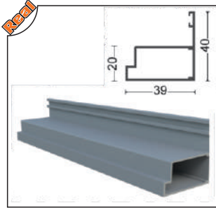
ISICM31-1009 Yan Kasa Profili Aluminum Side Profile (With PVC Seal)
