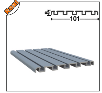
SRM-1003 Eşiksiz Alt Kasa Profili Without Treshold - Lower Frame Alm. Profile
