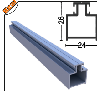
OPT-1014-50 Yan Dayama Profili Sidebar Profile
