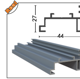
PRGLD-1006 Kollu Fıtil Karşılığı Contalı Esp.Handle Opposite Alm. Seal (With PVC Seal)
