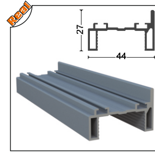
ISICM31-1010 Küçük h Fıtil Contalı Esp.Handle Seal (With PVC Seal)
